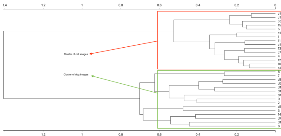
Fig. 4.31: Dendrogram
