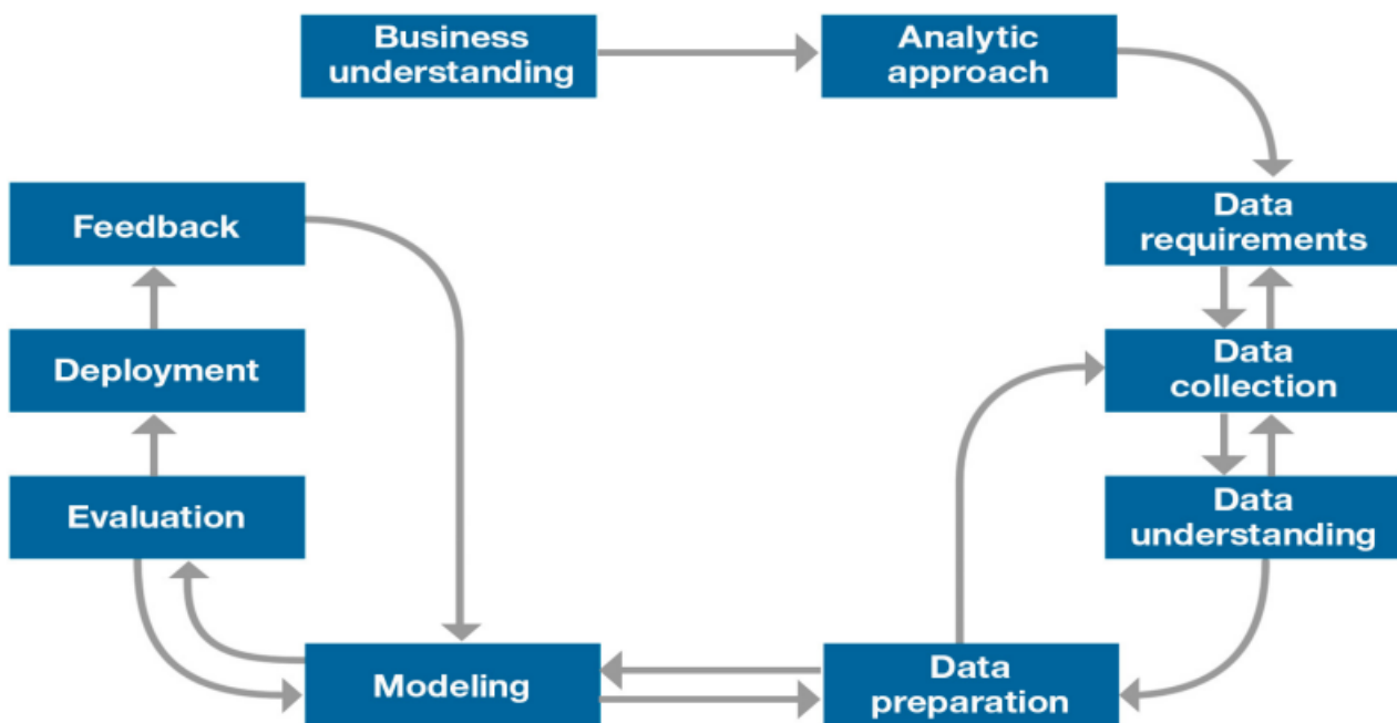
Figure 1. Foundational methodology for data science.
