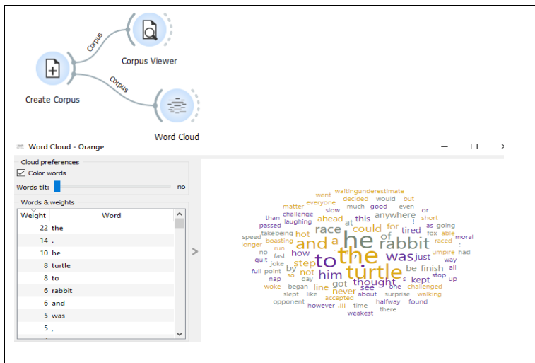
Fig. 4.36: Visualize word frequencies with cloud word
